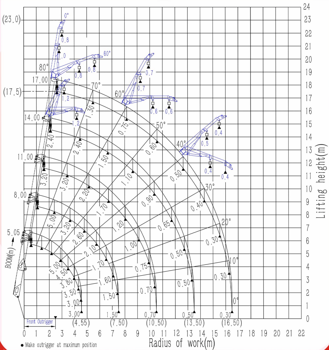
SPT499 Lifting Chart with Fly Jib
